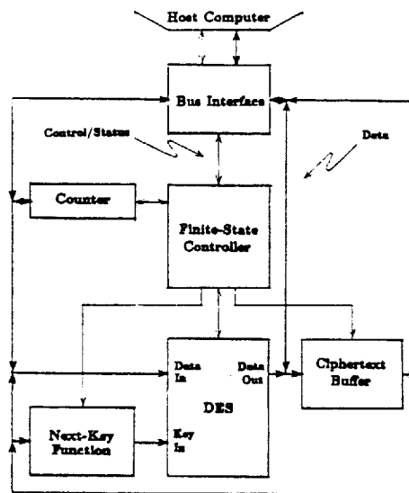
Figure 1: Block diagram of special-purpose hardware
