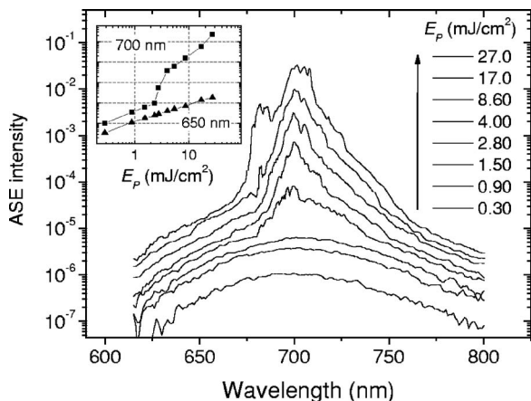
FIG. 1. Amplified spontaneous emission (ASE) spectra for different energy densities E_p for the waveguide impregnated with a 10^{-4}M Nile blue ethanolic solution. The inset refers to the integrated ASE intensities of two different windows centered at 700 nm (squares) and at 650 nm (triangles) vs pump energy.
