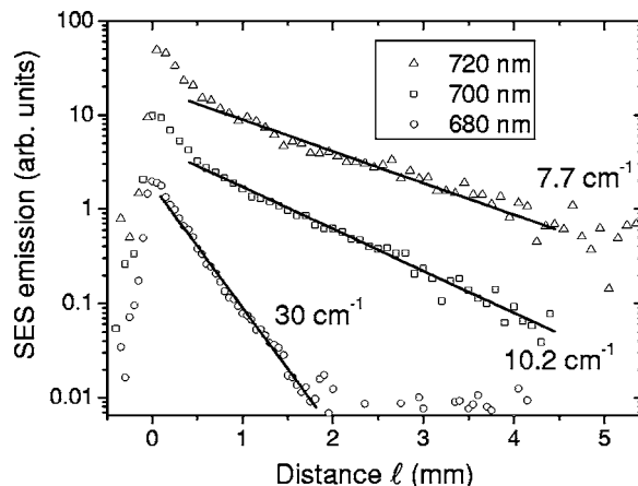
FIG. 2. Guided photoluminescence (PL) vs distance \ell between the spot and the waveguide edge (SES measurement). The wavelengths are 720 nm (triangles), 700 nm (squares), and 680 nm (circles). The exponential decay fits are shown with a solid line, and the loss value labels each line.
