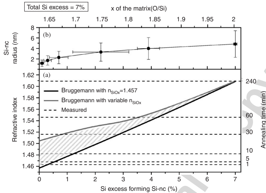
Fig. 1. Panel (a): two-component Bruggemann calculation using \text{SiO}_2 refractive index of 1.457 (black line) and using the refractive indices of \text{SiO}_x found in literature as a function of x (gray line). Dashed lines correspond to the measured refractive indices of the different samples. Panel (b) plots the dependence between the radius of Si-nc and the silicon excess forming part of Si-nc for a Si-nc density of 1\text{--}5 \times 10^{17} \text{ cm}^{-3} .
